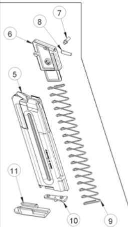
Assembly magazine
