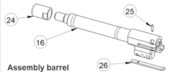
Assembly barrel
